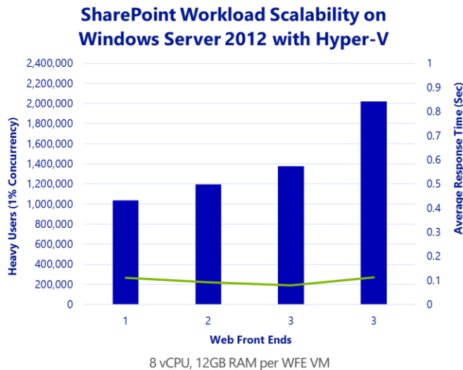
Figure 9 – Graph of virtualized SharePoint 2013 scalability with increased demand
