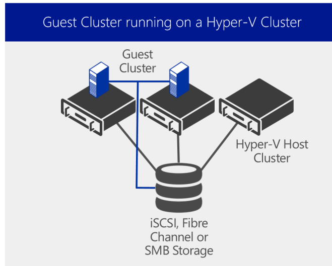
Figure 14 – A Guest Cluster running on a Hyper-V Cluster
