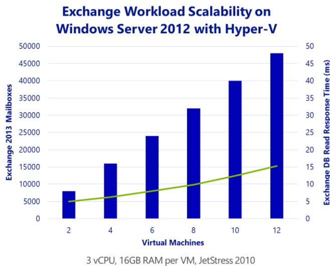
Figure 7 – Graph of virtualized Exchange 2013 scalability
