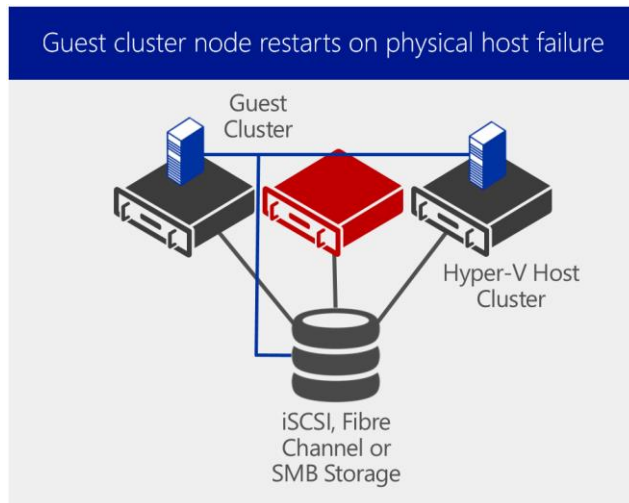
Figure 15 – A Guest Cluster running on a Hyper-V Cluster that has a single node failure
