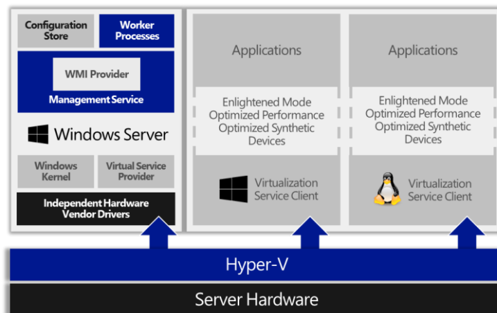
Figure 11 – Architectural view of Linux running enlightened on Hyper-V
