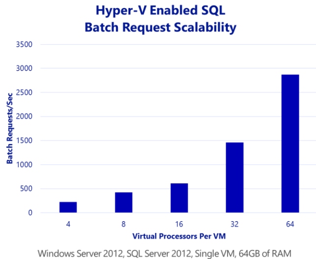
Figure 5 – Graph of a Hyper-V Enabled SQL Batch Request Scalability
