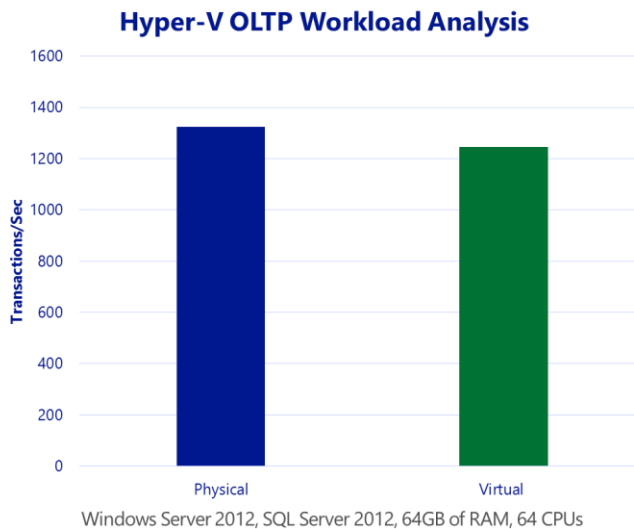
Figure 6 – Graph of a Hyper-V OLTP Workload Analysis
