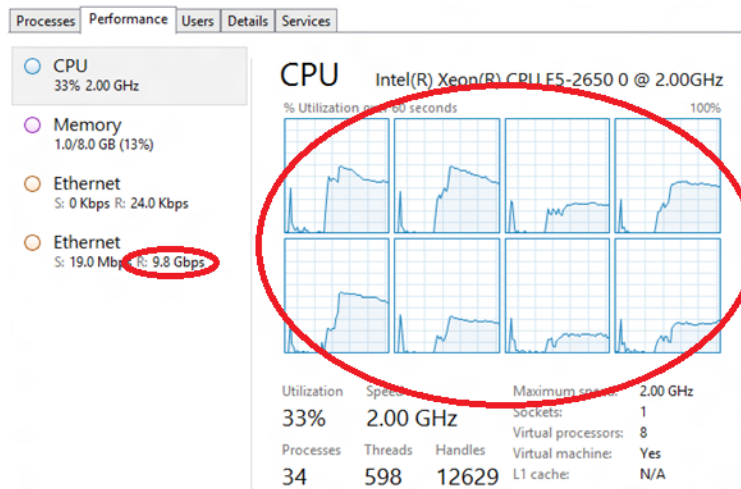
Figure 2 – vRSS enables all vCPUs to be utilized to process network traffic
