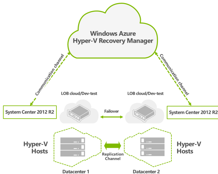
Figure 17 – Windows Azure Hyper-V Recovery Manager
