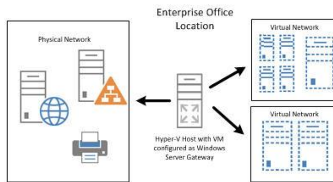
Figure 13 – Single location, with the WSG being used to connect VMs with physical infrastructure
