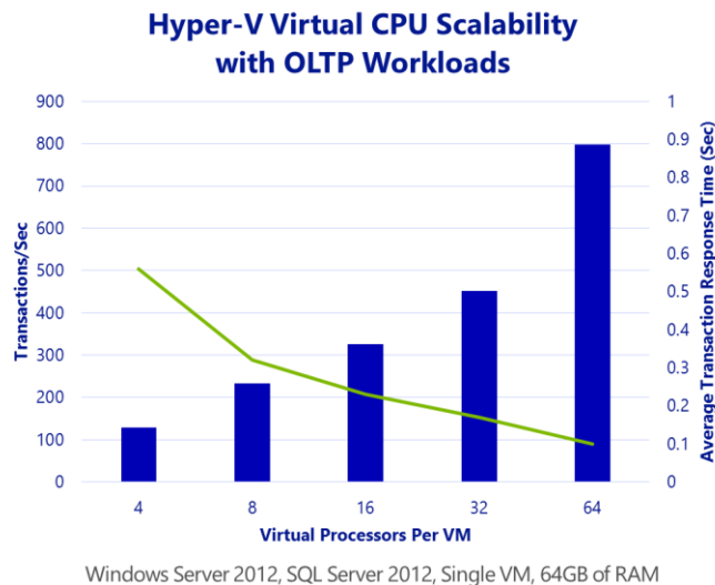
Figure 4 – Graph of a Hyper-V Virtual CPU Scalability with OLTP Workloads
