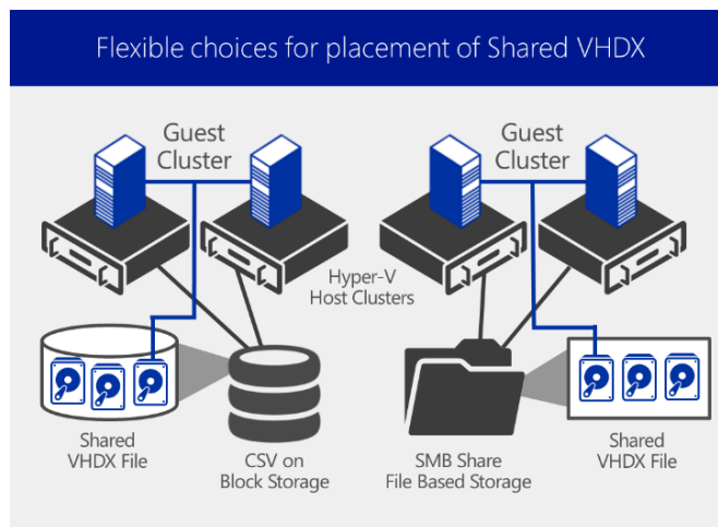
Figure 16 – A Guest Cluster using Shared VHDX on CSV/SMB Storage
