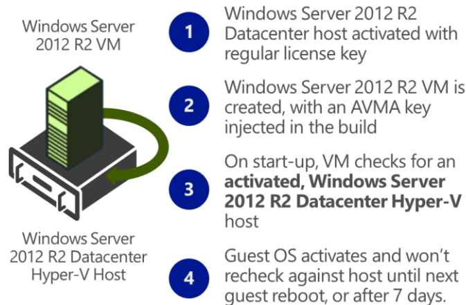
Figure 20 – Automatic VM Activation
