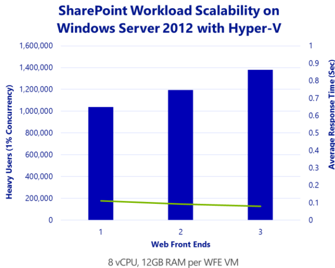
Figure 8 – Graph of virtualized SharePoint 2013 scalability
