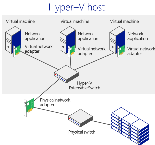
Figure 10 – Network with Hyper-V Extensible Switch
